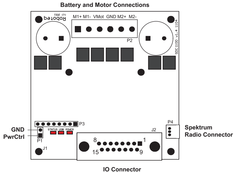
FIGURE 8. Controller layout
