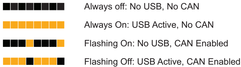
FIGURE 9. Communication LED
