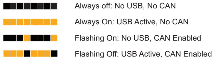
FIGURE 9. Communication LED
