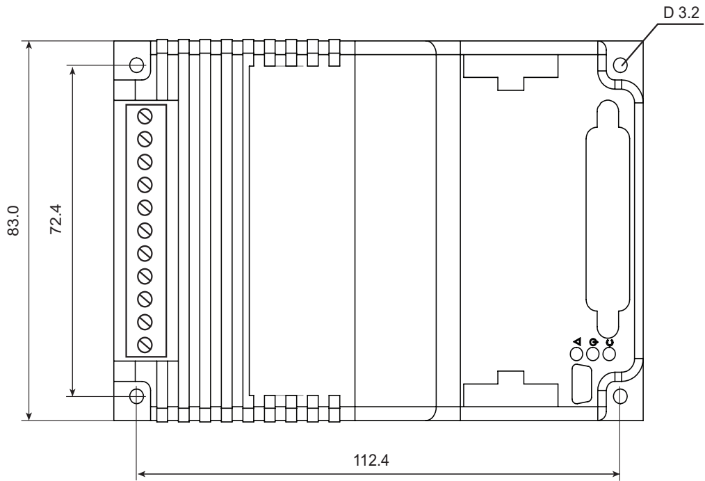
FIGURE 11. SDC3260 Top View and Dimensions
